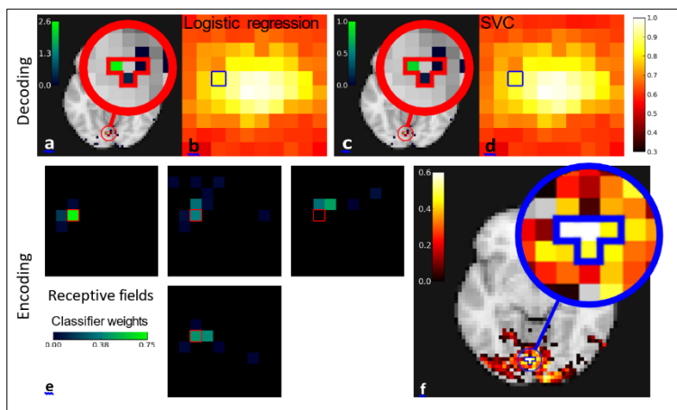
Fig 2: Miyawaki results. Top (Decoding): (a)/(c) classifier weights from logistic regression/SVM; (b)/(d) reconstruction accuracy per pixel. Bottom (Encoding): (e) receptive fields and (f) reconstruction accuracy by stimulus pixel.
